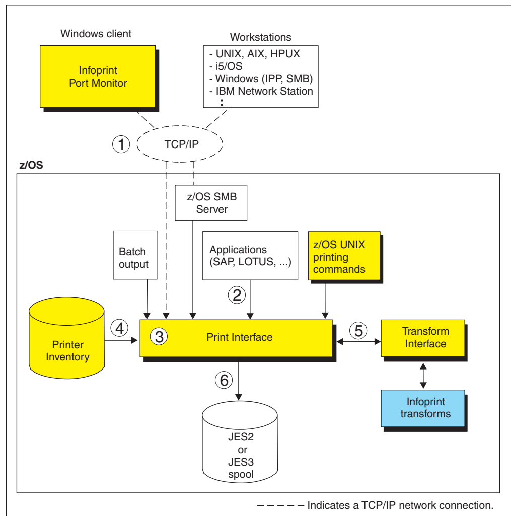
Figure 3. Print Interface system diagram
