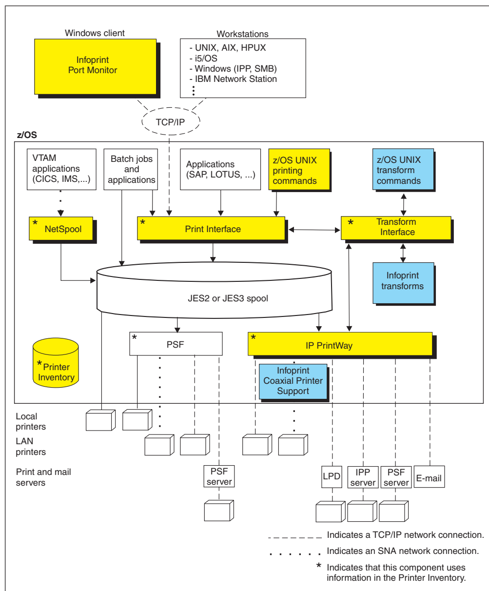
Figure 1. Infoprint Server system diagram
