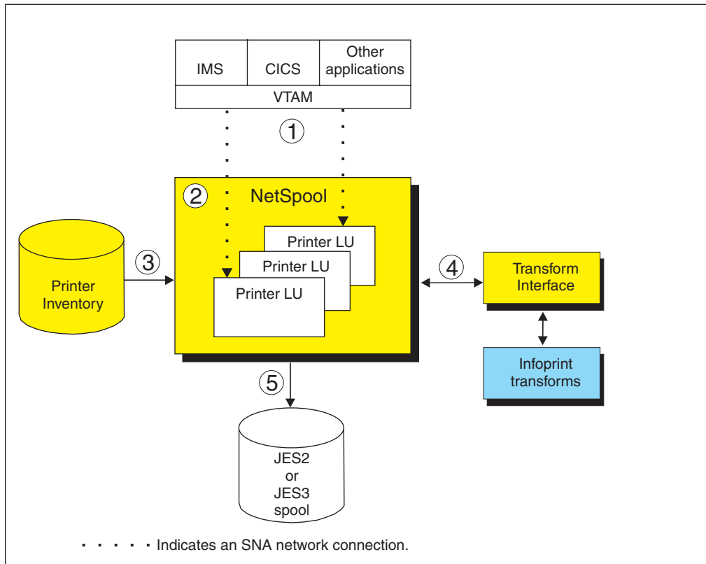
Figure 6. NetSpool system diagram
