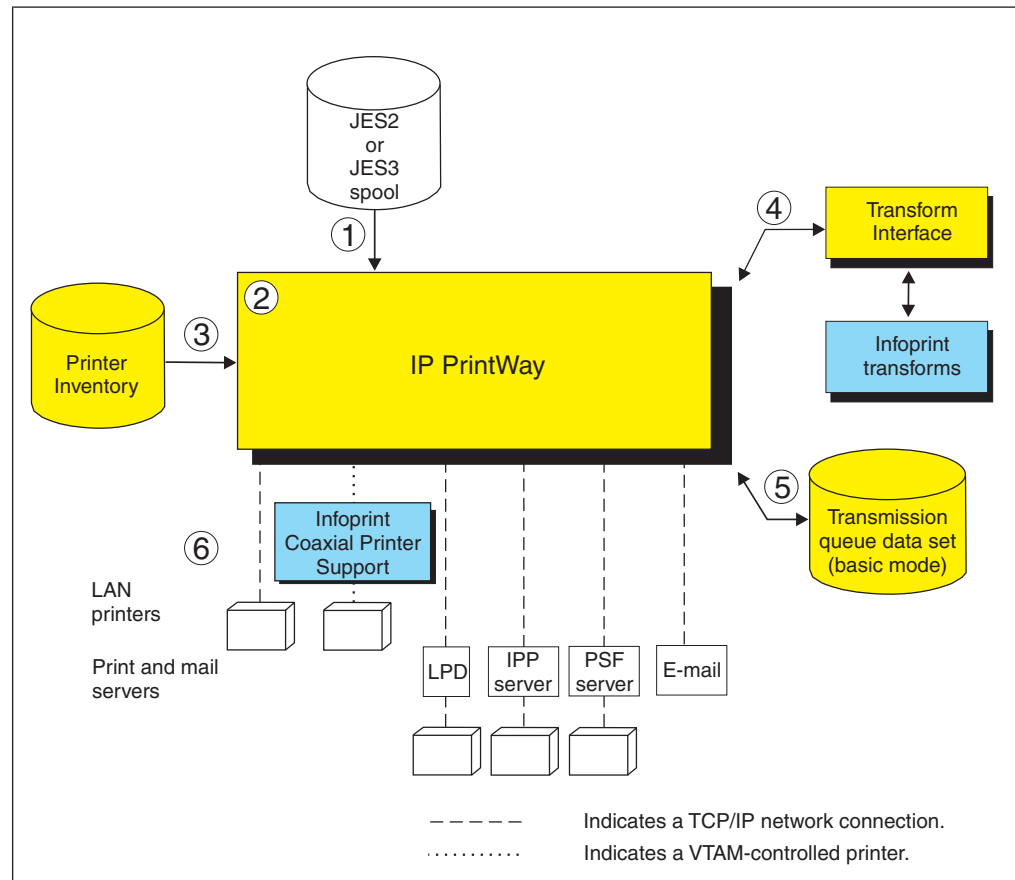
Figure 7. IP PrintWay system diagram
